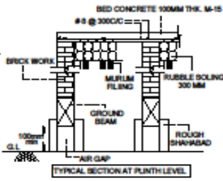
TYPICAL SECTION AT PLINTH LEVEL
