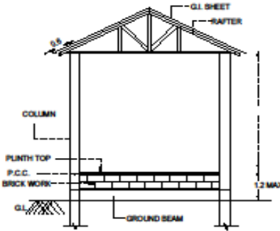
ground beam
