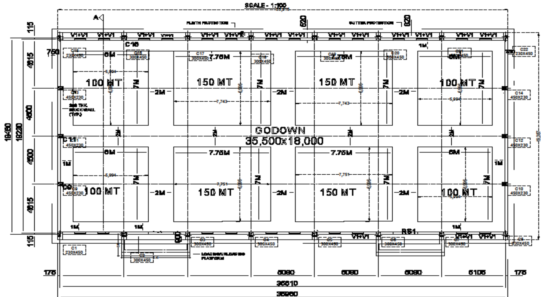
PLAN SCALE - 1:100
