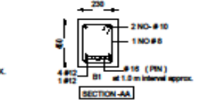
BEAM AT GROUND LEVEL
