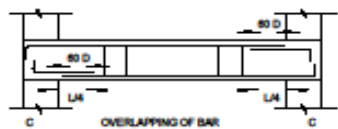
OVERLAPPING OF BAR
